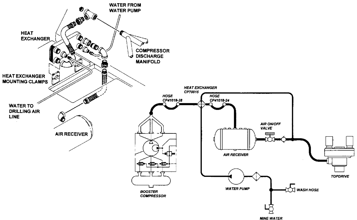
5200 DRILL HEAT EXCHANGER RETROFIT AIR SCHEMATIC
